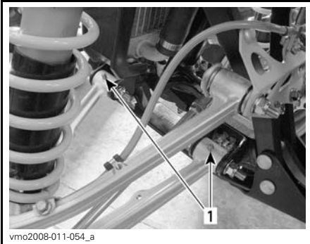
TYPICAL — LOWER SUSPENSION ARM
