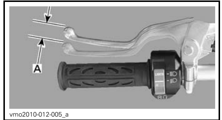
CLUTCH LEVER — PROPER ADJUSTMENT A. 10 mm to 15 mm (.39 in to .59 in)
