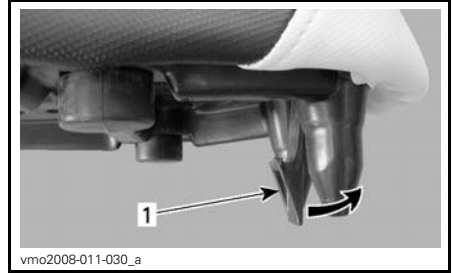
1. Seat latch
