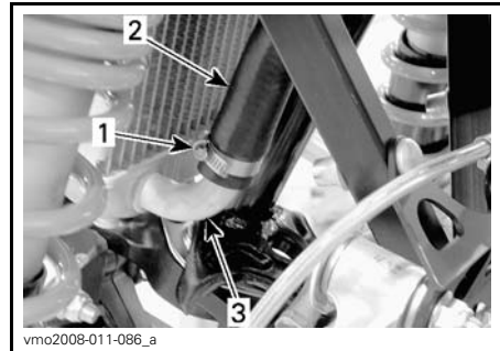
1. Gear clamp 2. Outlet hose 3. Radiator
