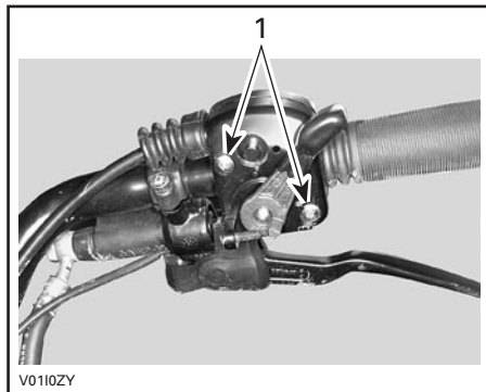
1. Remove screws
