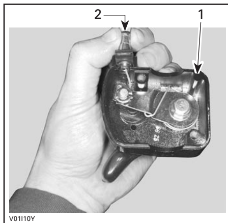
1. Throttle lever housing 2. Throttle cable
