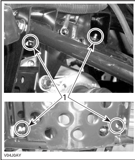
1. Grease fittings
