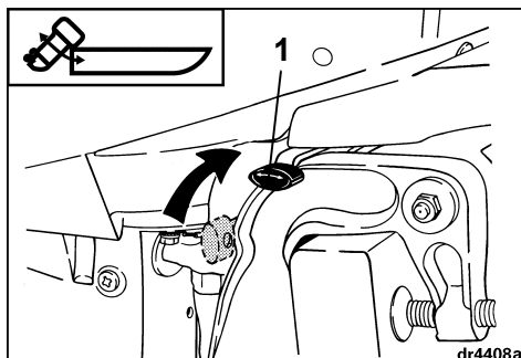
1. Tilt/vaarhendel – TILT-stand
