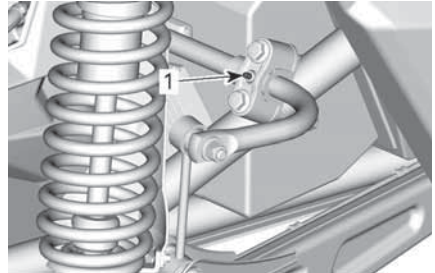
TYPICAL - REAR STABILIZER BAR
