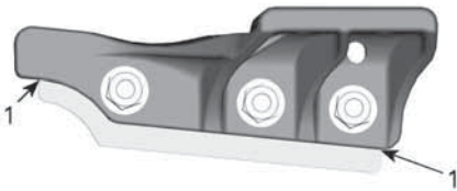
1. Wear limit
