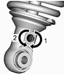
REBOUND DAMPING - BOTTOM OF SHOCK ABSORBER
