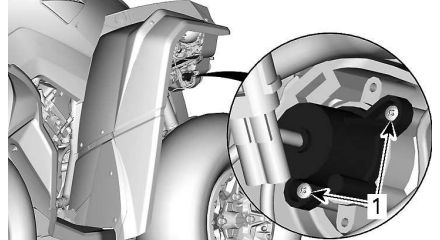
FRONT TURN SIGNAL LIGHT
