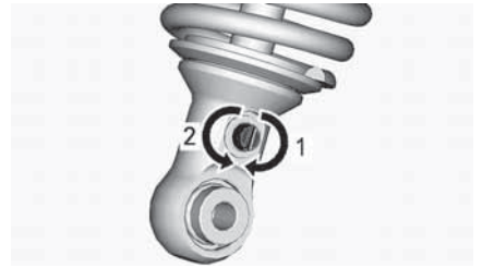
REBOUND DAMPING - BOTTOM OF SHOCK ABSORBER
