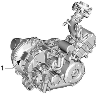
BACK OF 450 ENGINE
