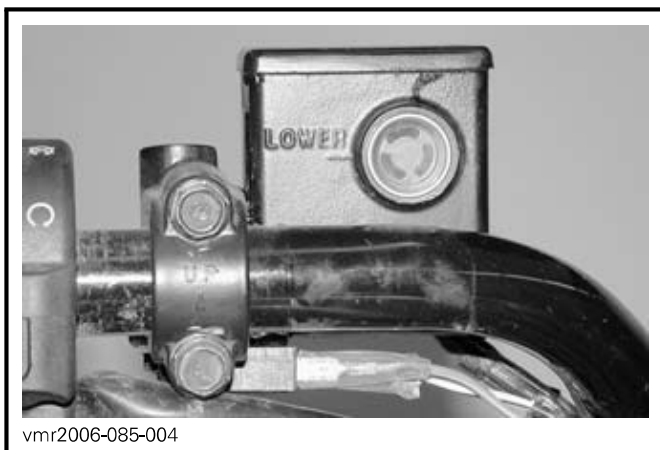
TYPICAL — LH REAR BRAKE FLUID RESERVOIR
