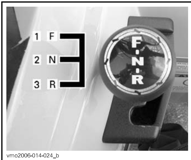
TRANSMISSION LEVER PATTERN
