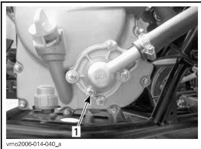
1. Cooling system drain plug
