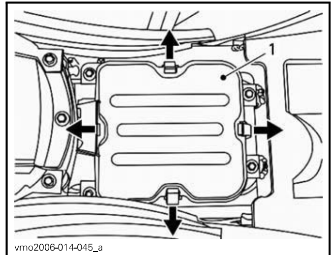
1. Air filter housing cover
