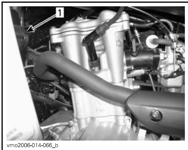
LH SIDE OF ENGINE 1. Air injection valve
