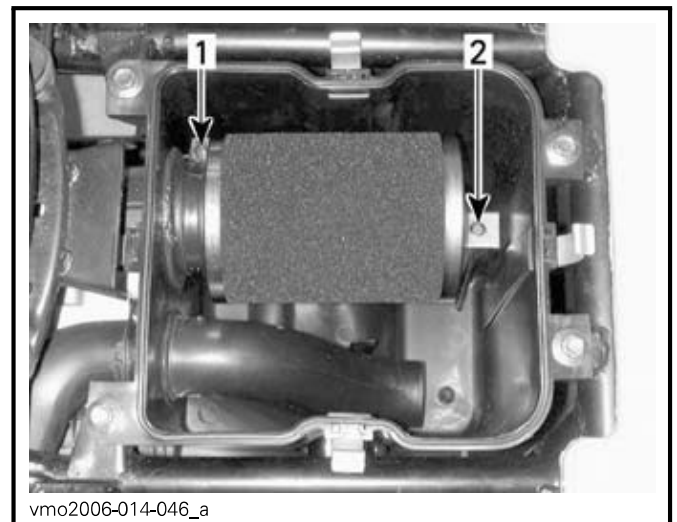
1. Clamp 2. Retaining screw
