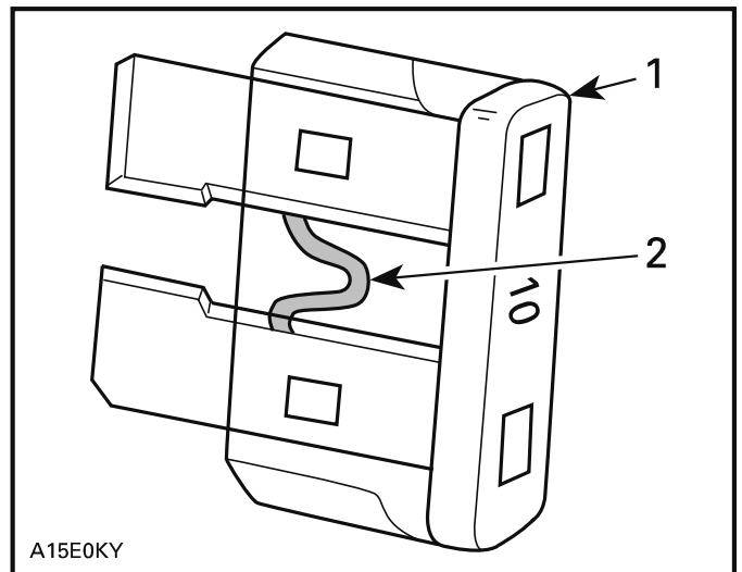
1. Fuse 2. Check if melted
