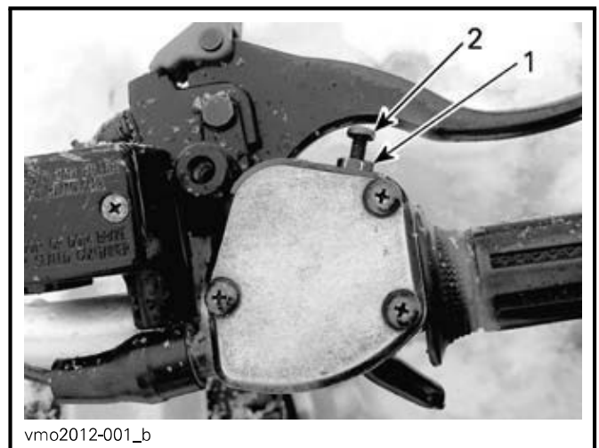
1. Lock nut 2. Speed limiter screw
