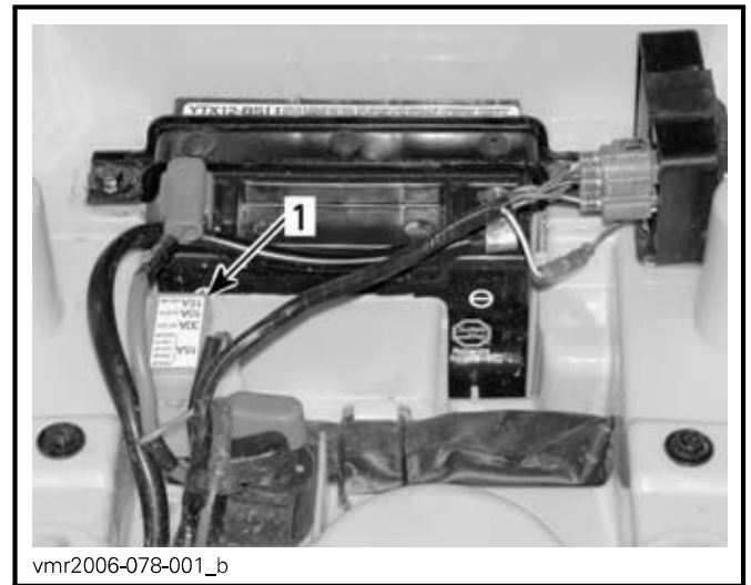
1. Fuse holder
