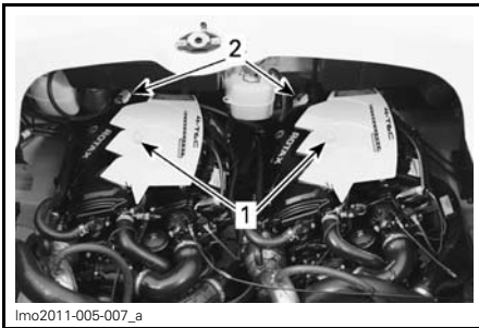
TYPICAL 1. Dipstick 2. Oil cap
