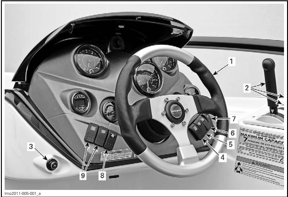
lmo2011-005-001_a COCKPIT VIEW
