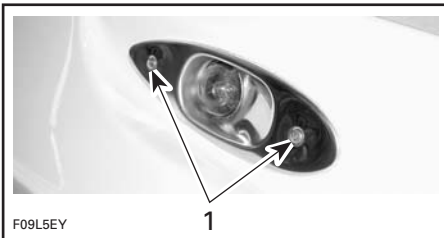
TYPICAL 1. Remove these screws
