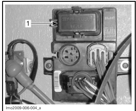
VEHICLE CONTROL MODULE (VCM) 1. Fuse cover
