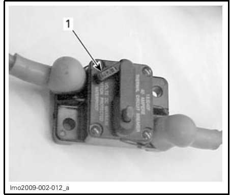
1. Reset lever in open (OFF) position
