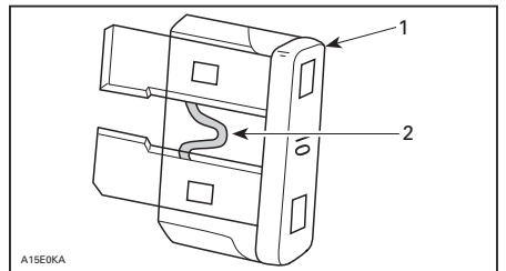
1. Fuse 2. Check if melted
