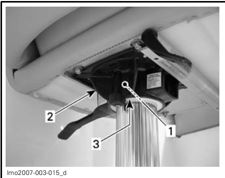
TYPICAL 1. Light film of grease 2. Casting hub 3. Cup
