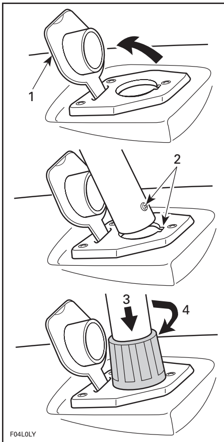
1. Bow eyelet
