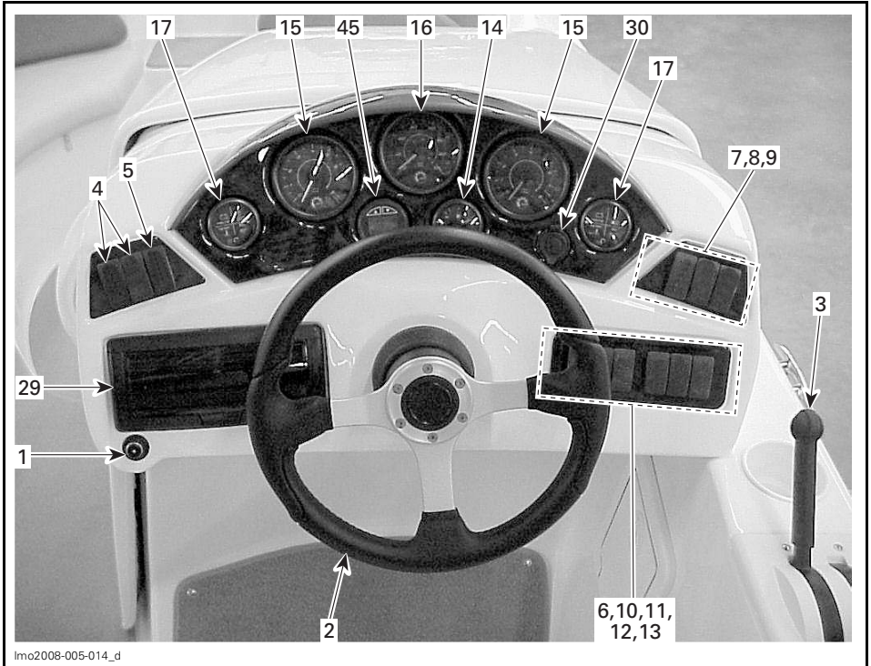
COCKPIT VIEW
