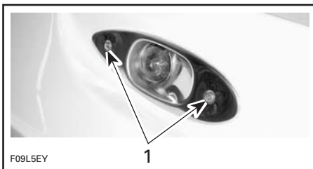
1. Remove these screws
