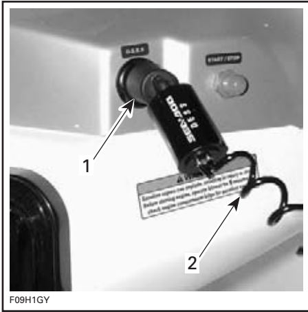
TYPICAL 1. DESS key installed on DESS post 2. Safety lanyard attached to operator
