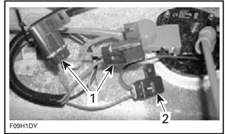
TYPICAL 1. Gauge interface fuses 2. Automatic bilge pump fuse
