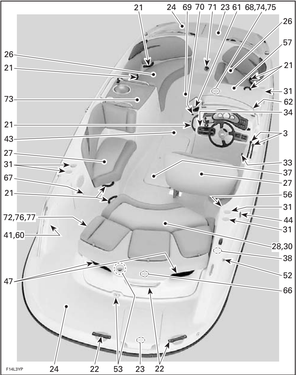
TYPICAL — 220 ISLANDIA SE
