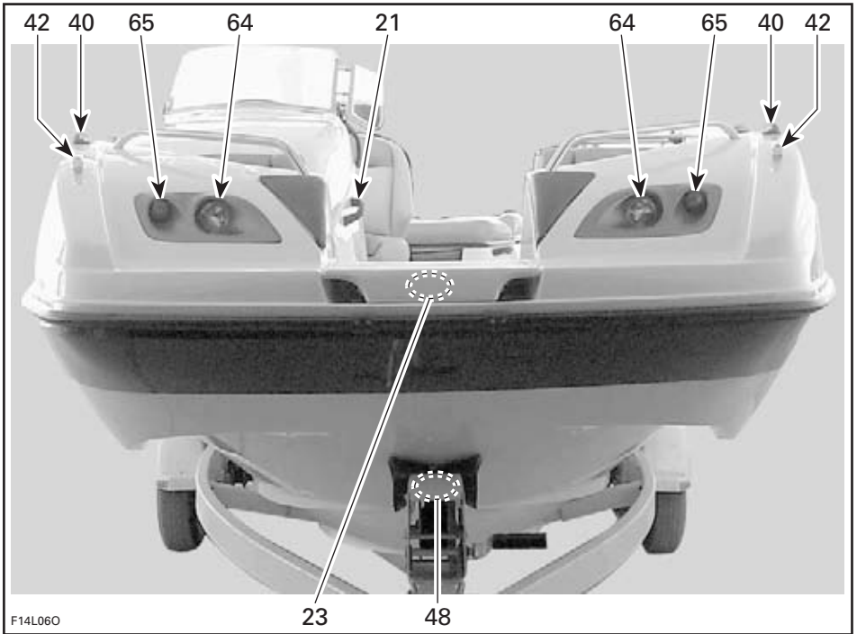
TYPICAL — FRONT VIEW — 220 ISLANDIA SE
