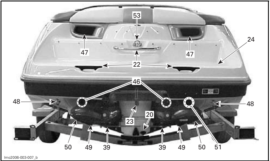
TYPICAL — REAR VIEW — 205 UTOPIA
