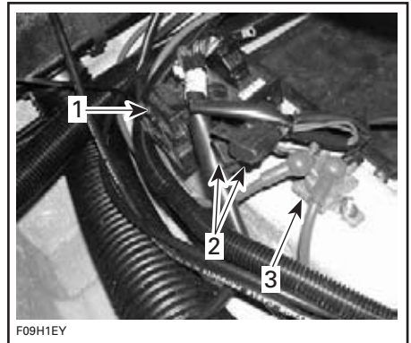
TYPICAL 1. Engine fuse block 2. Engine electrical system main fuses 3. Solenoid
