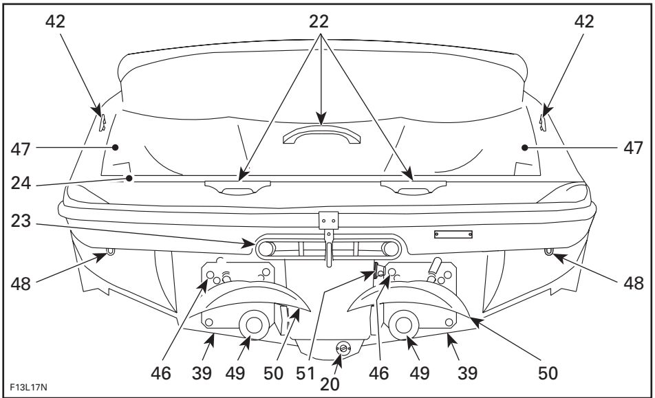
TYPICAL — REAR VIEW — 200 SPEEDSTER
