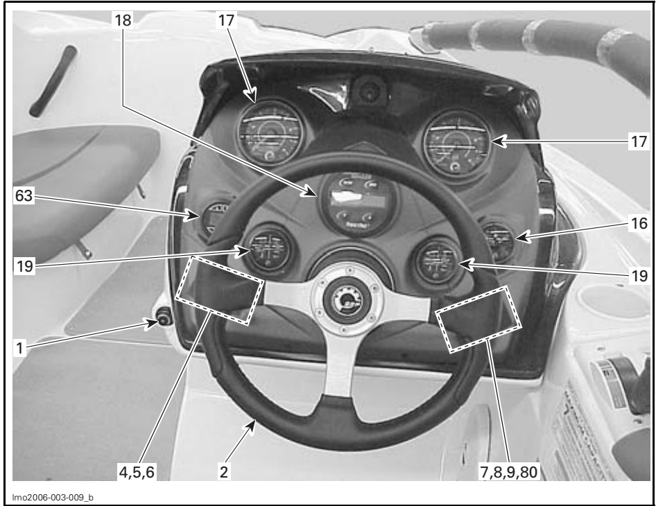
COCKPIT VIEW — 200 SPEEDSTER
