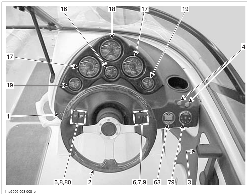
COCKPIT VIEW — 205 UTOPIA
