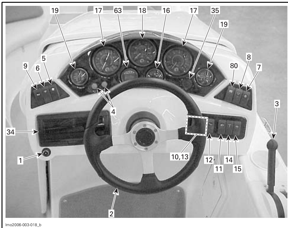
COCKPIT VIEW — 220 ISLANDIA SE
