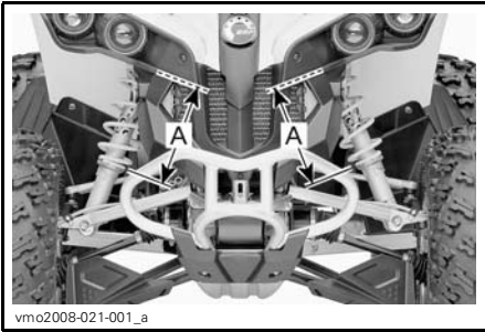
TYPICAL — PRELOAD ADJUSTMENT — FRONT
