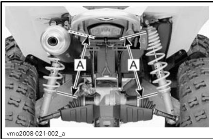
TYPICAL — PRELOAD ADJUSTMENT — REAR
