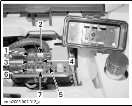
TYPICAL — FRONT FUSES LOCATION
