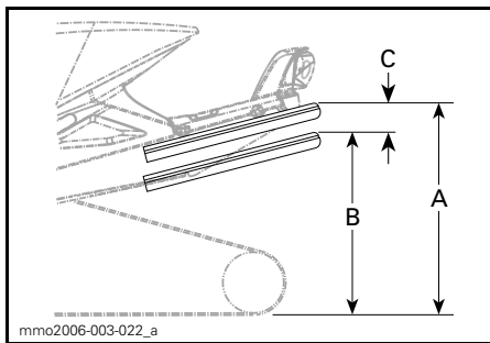
TYPICAL — PROPER ADJUSTMENT A. Suspension fully extended B. Suspension has collapsed with operator, passenger and load added C. Distance between dimension "A" and "B", see table below
