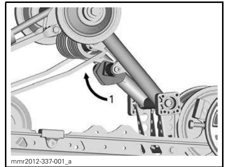
TYPICAL — LH SIDE 1. Adjust spring preload
