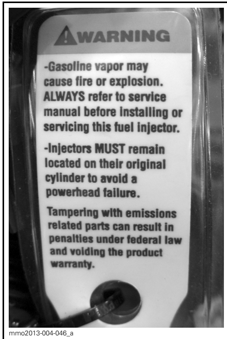
mmo2013-004-046_a ON FUEL INJECTORS - E-TEC ONLY
