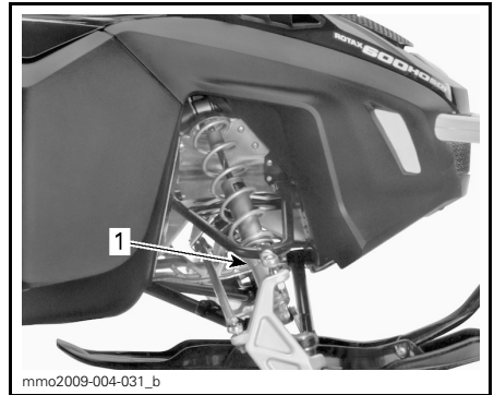
TYPICAL - CAM TYPE PRELOAD 1. Adjustment cam
