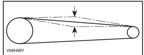
FREE-PLAY: 44 TO 57 MM (1-3/4 TO 2-1/4 IN)
