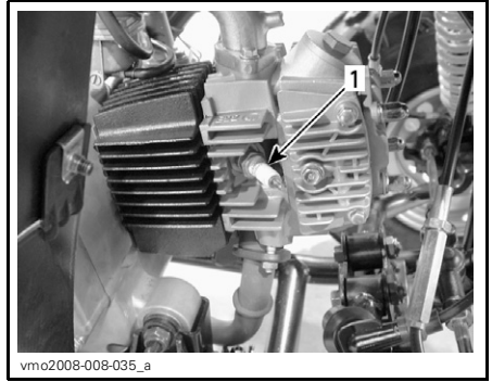
UNSCREW SPARK PLUG ONE TURN 1. Spark plug
