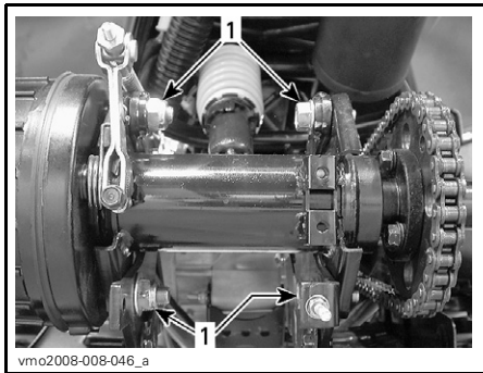
TYPICAL — REAR AXLE 1. Locking bolts
