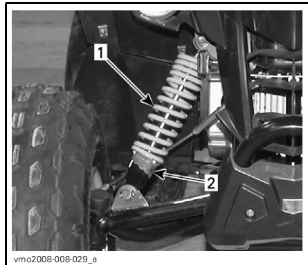
DS 70/DS 90 — FRONT SUSPENSION
