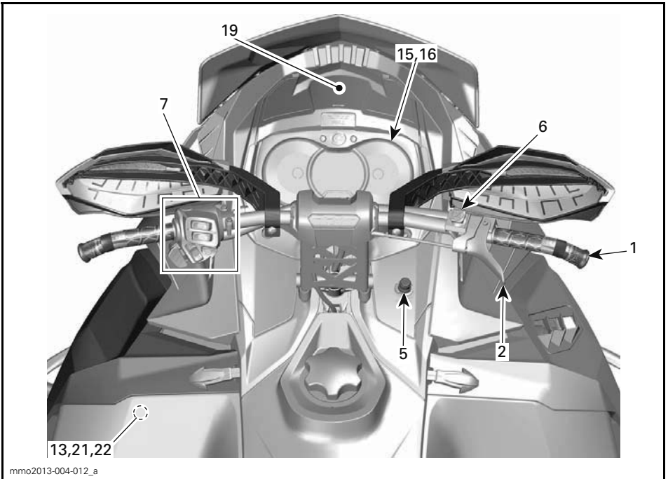
TYPICAL - MX Z AND RENEGADE MODELS
