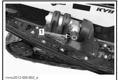
TYPICAL - rMOTION WITH QUICK ADJUST KNOB - RH SIDE
