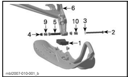
PARTS LAYOUT - LH SIDE SHOWN
