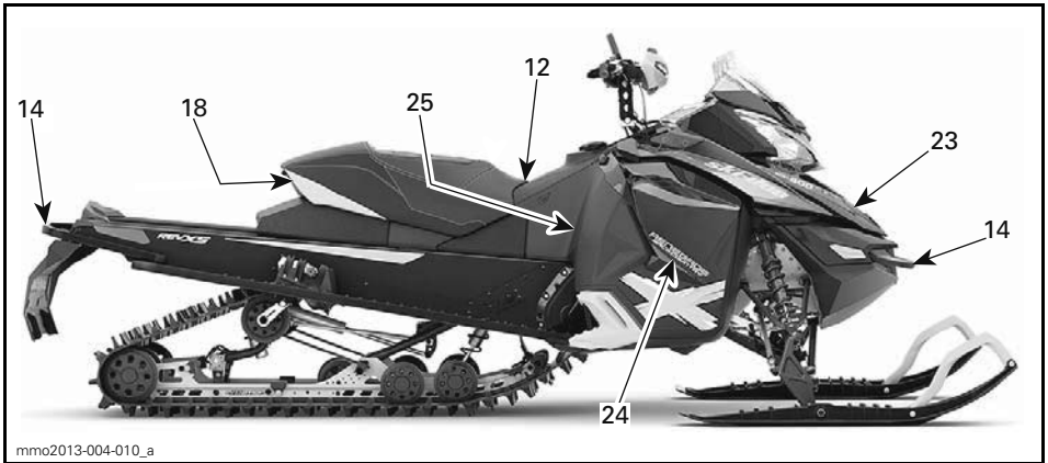
TYPICAL - MX Z AND RENEGADE MODELS
