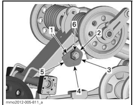
rMOTION WITHOUT QUICK ADJUST KNOB - RH SIDE
