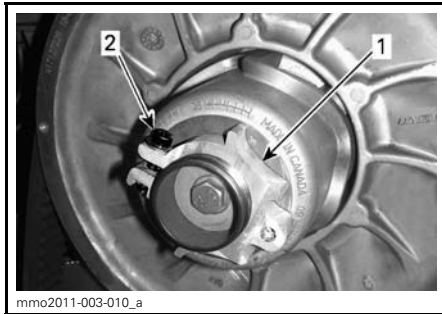
ALUMINUM ADJUSTER HUB 1. Adjuster hub 2. Clamping bolt
