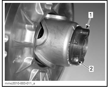
PLASTIC ADJUSTER HUB 1. Adjuster hub 2. Clamping bolt
