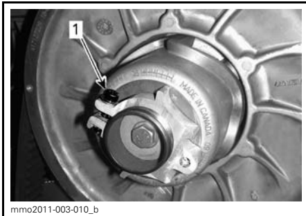
1. Clamping bolt
