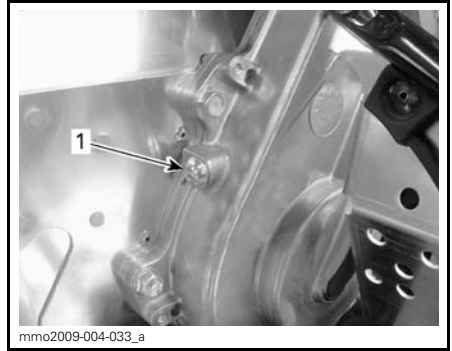
1. Check plug
