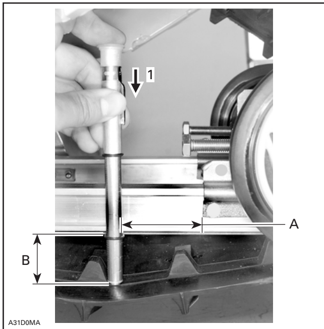
1. Belt tension tester
