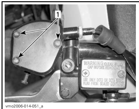
1. Remove screws
