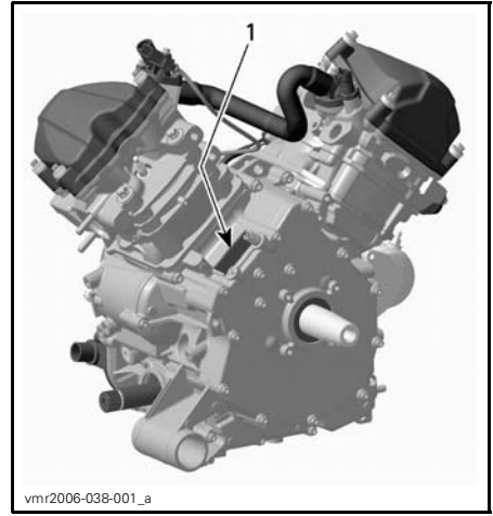
TYPICAL — ENGINE SERIAL NUMBER LABEL 1. EIN (Engine Identification Number)
