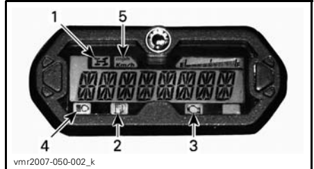
1. 4WD indicator lamp 2. Low fuel level indicator lamp 3. Check engine indicator lamp 4. High beam indicator lamp 5. MPH or km/h indicator lamp
