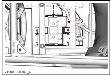
1. Battery holder 2. Battery 3. Battery holder retaining screw(s)
