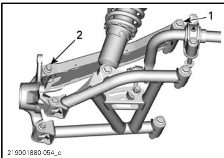
1. Elastic flange nut M12 2. Hexagonal flanged elastic nut M10
