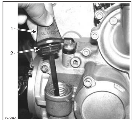
RH SIDE OF ENGINE 1. Dipstick 2. O-ring
