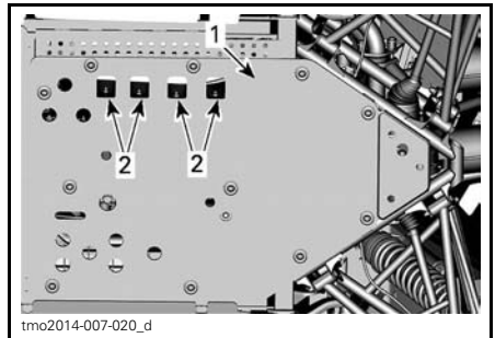
TYPICAL 1. Central skid plate 2. Access holes
