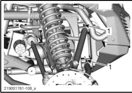
219001761-108_a TYPICAL - FRONT SUSPENSION 1. Grease fittings
