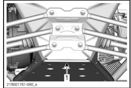
TYPICAL - REAR OF VEHICLE 1. Hydraulic jack position
