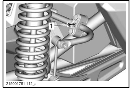
219001761-112_a TYPICAL - REAR STABILIZER BAR 1. Grease fitting
