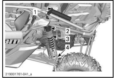
TYPICAL - MAVERICK X3 MAX X RS MODELS - REAR SUSPENSION
