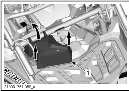
1. Service cover
