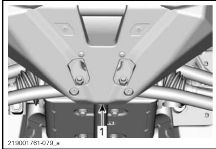
TYPICAL - FRONT OF VEHICLE 1. Hydraulic jack position
