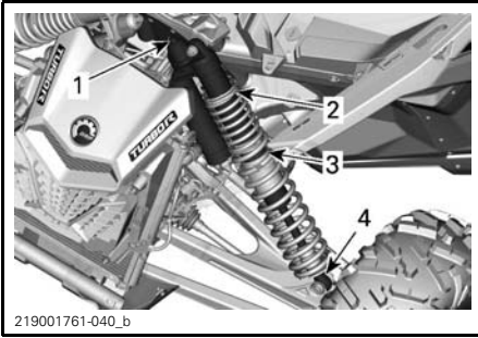
TYPICAL - MAVERICK X3 MAX X DS AND X RS MODELS - FRONT SUSPENSION
