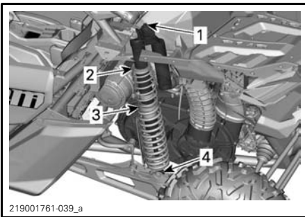
TYPICAL - MAVERICK X3 MAX X DS MODELS - REAR SUSPENSION
