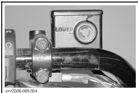
ACHTERREM-VLOEISTOFRESERVOIR LINKS
