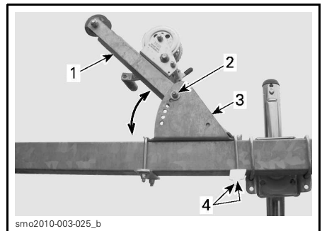
1. Winch arm 2. Winch arm adjustment bolt 3. Winch support 4. Front U-bolt nuts
