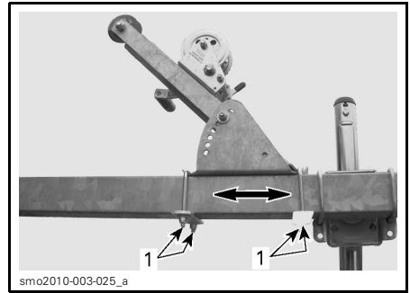
1. Winch support U-bolts nuts
