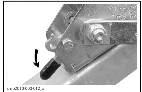
smo2010-003-012_a SET WINCH TO "UNWIND"
