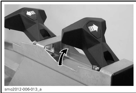
smo2012-006-013_a PULL HANDLE UP (SEA-DOO MOVE II)
