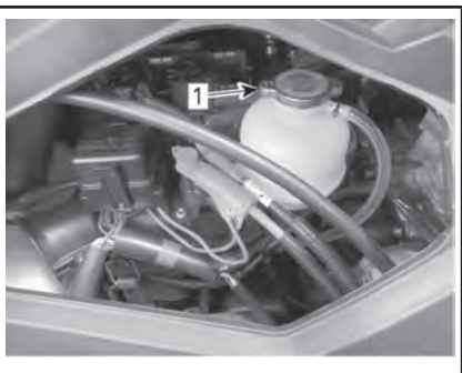
1. 膨胀箱盖
