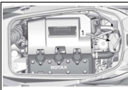
1. Expansionskärllets lock
