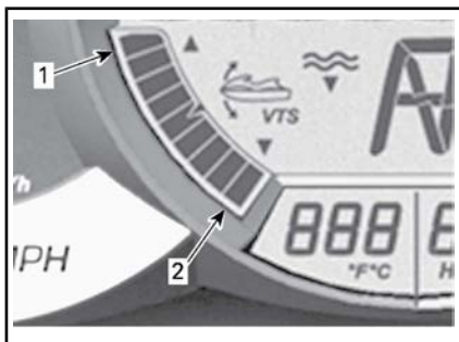
INFO-CENTER — VTS-POSITIONSANZEIGE
