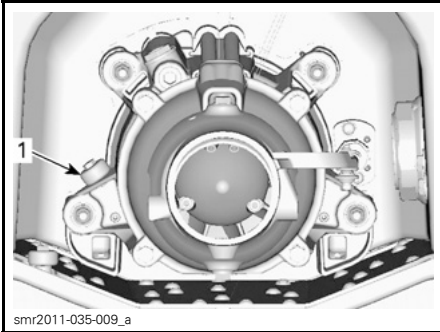
1. Offeranodens placering
