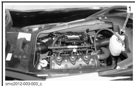
1. Expansionskärllets lock
