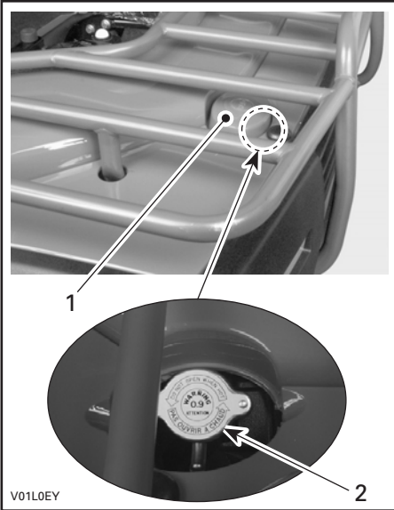
1. Protector cap 2. Radiator cap
