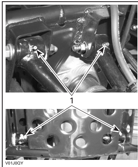
1. Grease fittings
