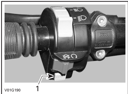
1. Start button
