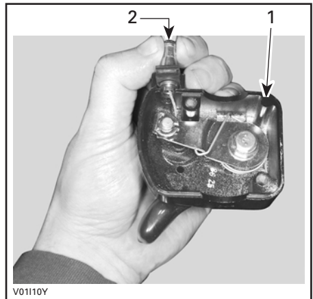
1. Throttle handle housing 2. Throttle cable
