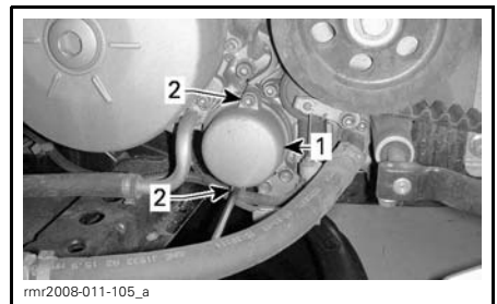
TYPICAL 1. Oil filter cover 2. Cover screws
