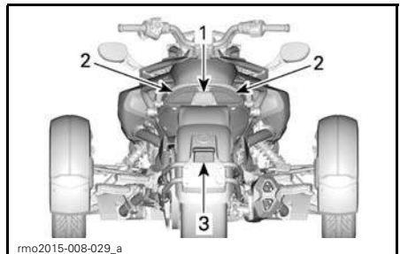
LIGHTS LOCATION — REAR OF VEHICLE — NORTH AMERICAN MODELS
