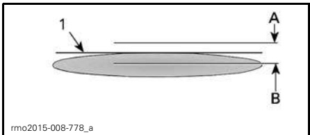
TYPICAL - HEADLIGHT REFLECTION ON TEST SURFACE (SINGLE HEADLAMP) 1. Top line A. Mark at 644 mm (25-23/64 in) above ground B. Mark at 554 mm (21-13/16 in) above ground
