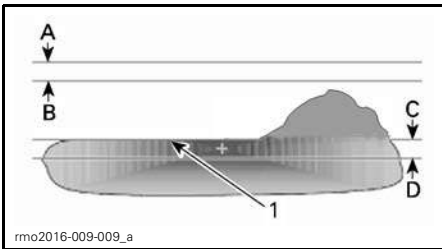
HEADLIGHT REFLECTION ON TEST SURFACE — LOW BEAM (SINGLE HEADLAMP)
