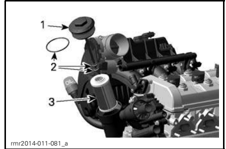
1. Oil filter cover 2. O-rings 3. Oil filter
