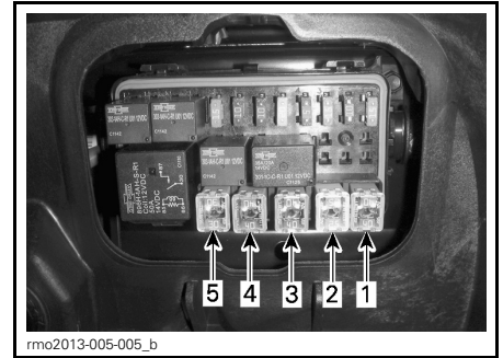
JCASE FUSES - LEFT FUSE BOX
