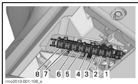
FUSES LOCATED UNDER THE SEAT
