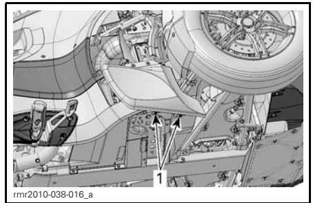
1. Push-in clips
