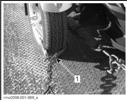
TYPICAL FRONT WHEELS ATTACHMENT — METHOD 1
