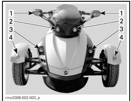
LIGHTS LOCATION — FRONT OF VEHICLE 1. Turn signal light 2. Headlight — high beam 3. Headlight — low beam 4. Position light
