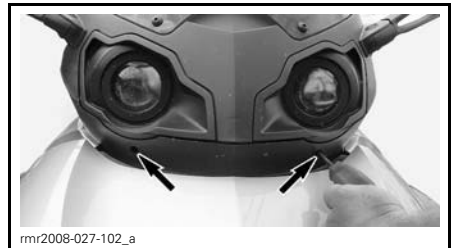
ADJUSTMENT SCREWS
