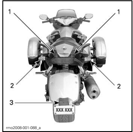
LIGHTS LOCATION — REAR OF VEHICLE
