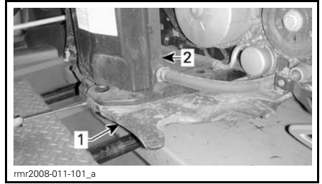
1. Bottom plate 2. Oil tank
