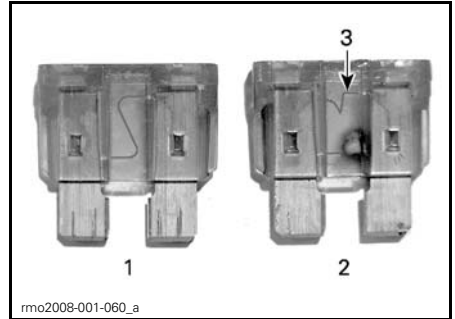
FUSE UNDER THE SERVICE COVER
