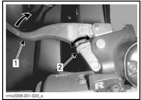
CLUTCH LEVER ADJUSTMENT
