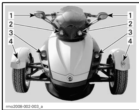
LIGHTS LOCATION — FRONT OF VEHICLE 1. Turn signal light (p. 113) 2. Headlight — high beam (p. 112) 3. Headlight — low beam (p. 111) 4. Position light (p. 115)
