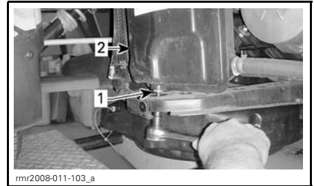
1. Reservoir drain plug 2. Oil tank
