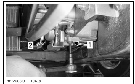
1. Engine oil drain plug 2. Oil filter cover
