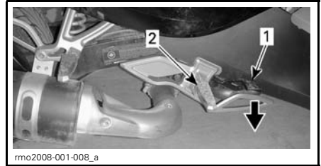
1. Brake pedal 2. Footpeg
