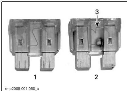
FUSE UNDER THE SERVICE COVER 1. Good fuse 2. Blown fuse 3. Melted filament
