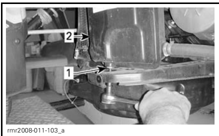
1. Reservoir drain plug 2. Oil tank
