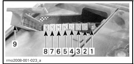
FUSES LOCATED UNDER THE SEAT
