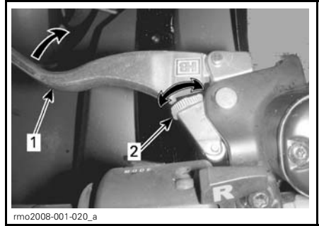
CLUTCH LEVER ADJUSTMENT
