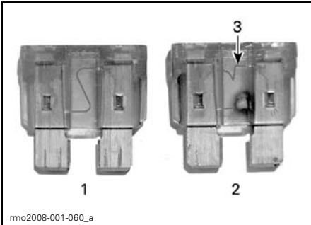
FUSE UNDER THE SERVICE COVER
