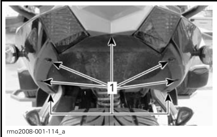
PANEL UNDER PASSENGER SEAT 1. 7 Torx screws location
