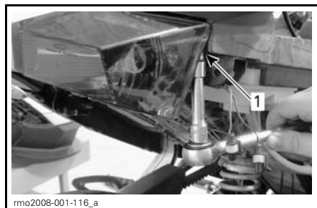
1. Removing Torx screw behind lens
