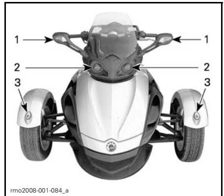
LIGHTS LOCATION – FRONT OF VEHICLE 1. Turn signal light (p. 112) 2. Headlight (p. 111) 3. Position light (p. 114)
