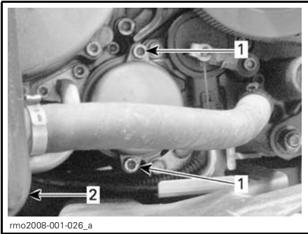
1. Oil filter cover screws 2. Bottom of oil tank
