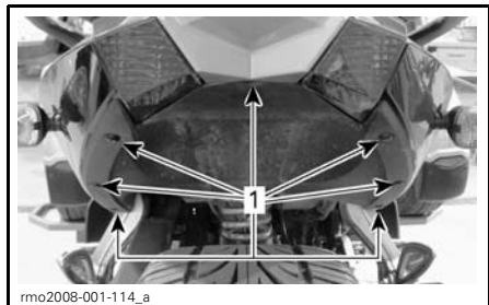
PANEL UNDER PASSENGER SEAT 1. 7 Torx screws location
