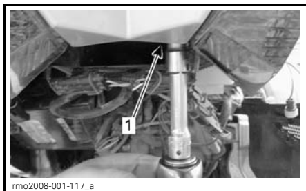
1. Removing Torx screw beside the lens
