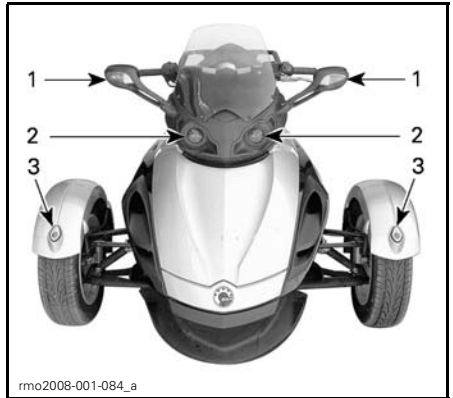
LIGHTS LOCATION – FRONT OF VEHICLE 1. Turn signal light (p. 108) 2. Headlight (p. 107) 3. Position light (p. 110)
