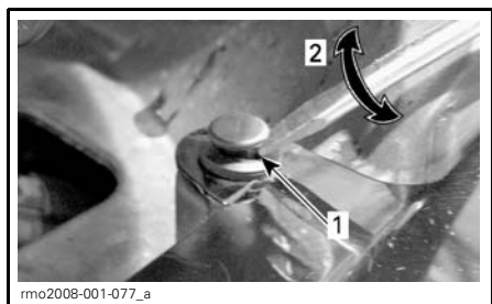
1. Flat head screwdriver under rivet head 2. Turn screwdriver 1/4 turn
