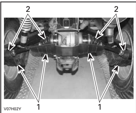
REAR OF VEHICLE 1. Drive shaft protectors 2. Drive shaft boots
