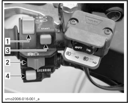
TYPICAL — MULTI-FUNCTION SWITCH
