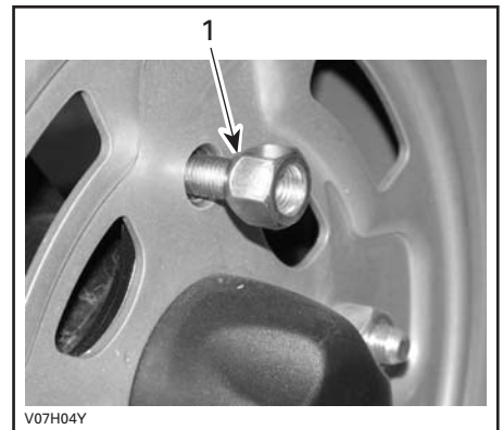
1. Taper side of nut
