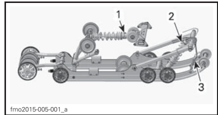
PPS-5900A AND PPS-6900A REAR SUSPENSION
