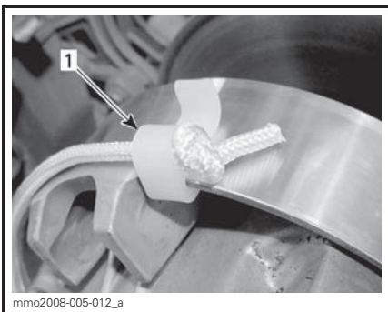
1. Clip installation location
