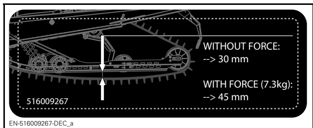
LABEL 2 - XTRIM SC MODELS
