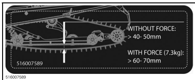
LABEL 2 - 49 RANGER PRO MODELS
